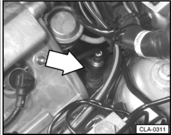
Z28 Oxygen Sensor (O2S) 2, heater (2.8 ltr. engine)
