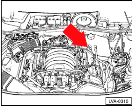
Z28 Oxygen Sensor (O2S) 2, heater (2.8 ltr. engine)
