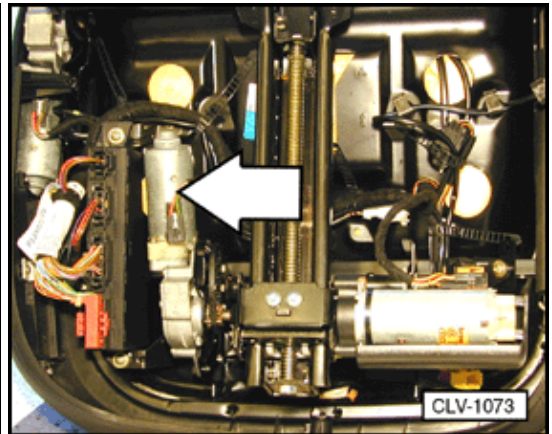
V29 Motor for front height adjustment, driver seat
