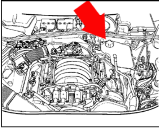
T3c 3-Pin Connector (2.8 ltr. engine)
