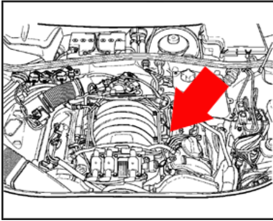
N83 Cylinder 5 Fuel Injector (2.8 ltr. engine)
