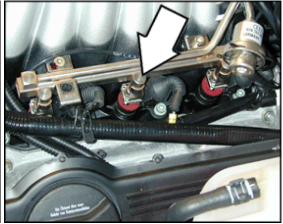
N83 Cylinder 5 Fuel Injector (2.8 ltr. engine)
