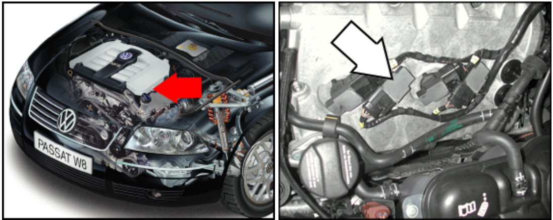
N324 Ignition Coil 6 with Power Output Stage (4.0 ltr. engine)
