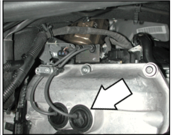
N205 Valve -1- for camshaft adjustment (4.0 ltr. engine)
