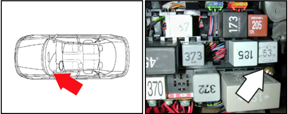
J434 Locking Relay for Starter (clutch pedal switch)
