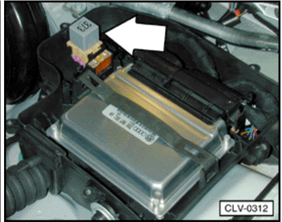
J299 Secondary Air Injection (AIR) pump relay (2.8 ltr. engine)
