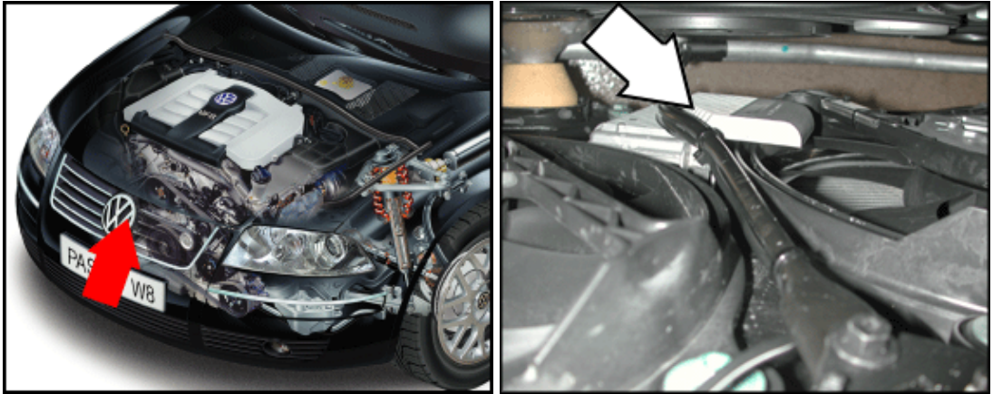
J293 Coolant FC (Fan Control) Control Module (4.0 ltr. engine)
