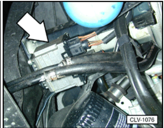
J293 Coolant FC (Fan Control) control module (All except 4.0 ltr. engine)
