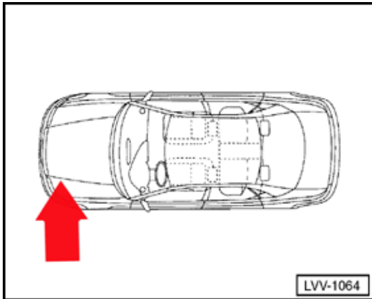
J293 Coolant FC (Fan Control) control module (All except 4.0 ltr. engine)
