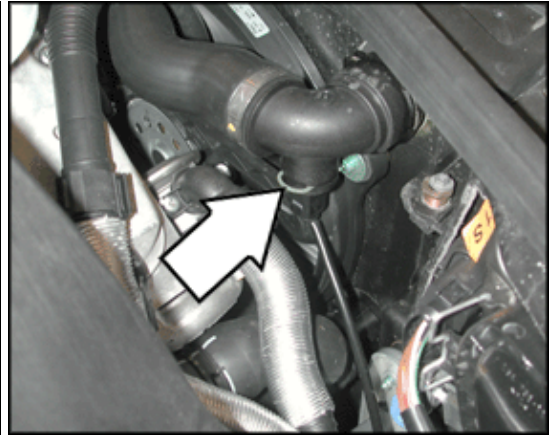
G83 Engine Coolant Temperature (ECT) Sensor (on Radiator) (4.0 ltr. engine)
