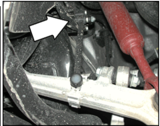
G78 Left Front Level Control System Sensor (4.0 ltr. engine)
