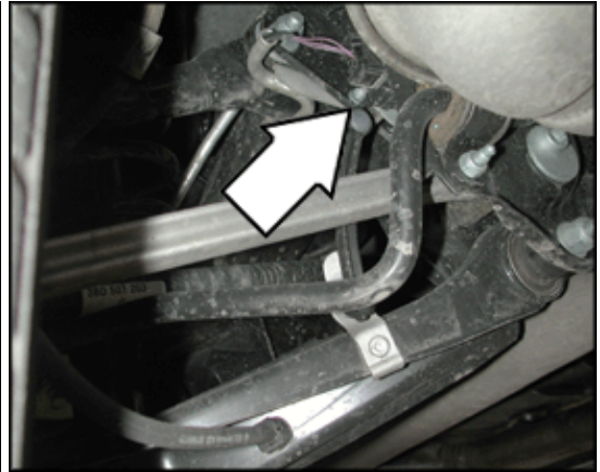
G76 Left Rear Level Control System Sensor (4.0 ltr. engine)
