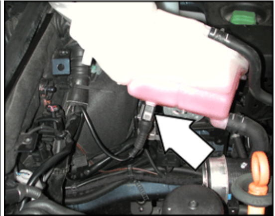
G32 Engine Coolant Level (ECL) Sensor (2.0 ltr. tdi engine)
