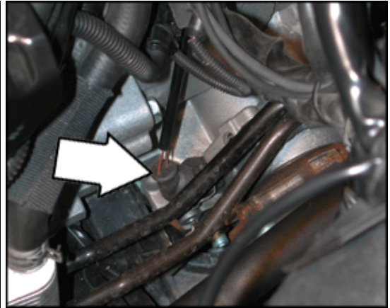
G22 Speedometer Vehicle Speed Sensor (VSS) (2.0 ltr. tdi engine)
