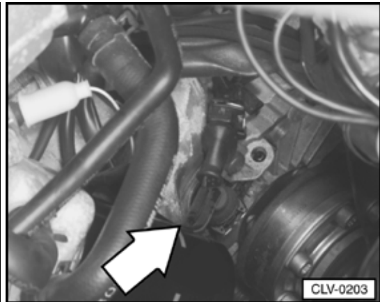
G22 Speedometer Vehicle Speed Sensor (VSS) (1.8 ltr. engine, 5-spd. 012)
