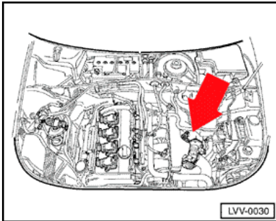
G22 Speedometer Vehicle Speed Sensor (VSS) (1.8 ltr. engine, 5-spd. 012)
