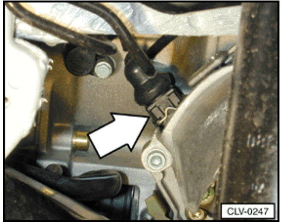
G22 Speedometer Vehicle Speed Sensor (VSS) (2.8 ltr. engine)
