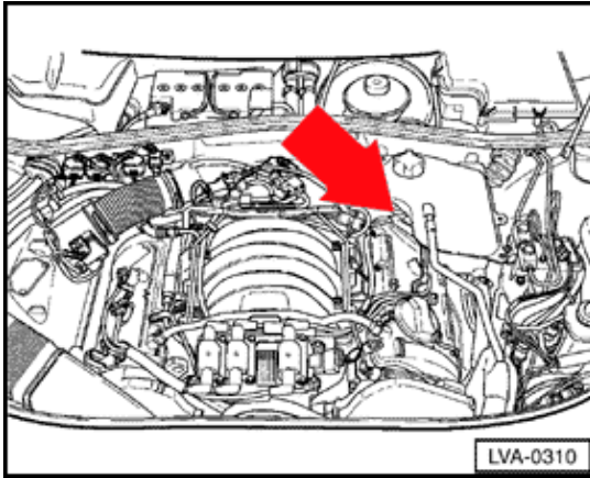
G163 Camshaft Position (CMP) sensor 1 (2.8 ltr. engine)
