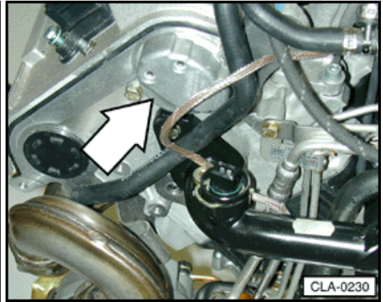
G163 Camshaft Position (CMP) sensor 1 (2.8 ltr. engine)
