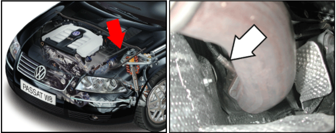
G131 Oxygen Sensor (O2S) 2 Behind Three Way Catalytic Converter (TWC) (4.0 ltr. engine)
