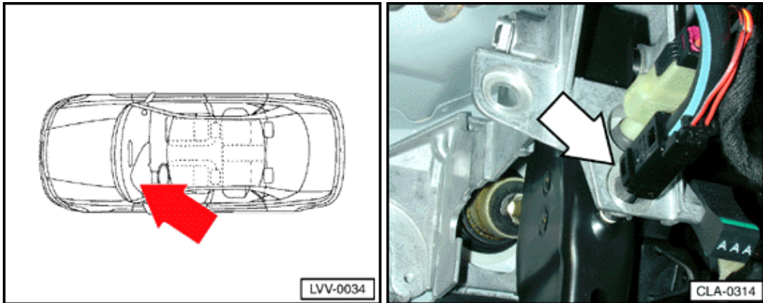
F47 Vacuum vent valve brake switch (through m.y. 1999)
