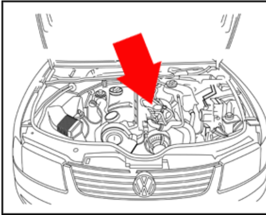
F1 Oil Pressure Switch (2.0 ltr. tdi engine)
