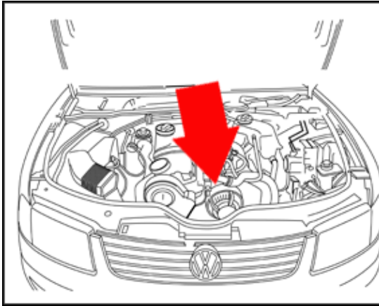
C1 Voltage Regulator (VR) (2.0 ltr. tdi engine)
